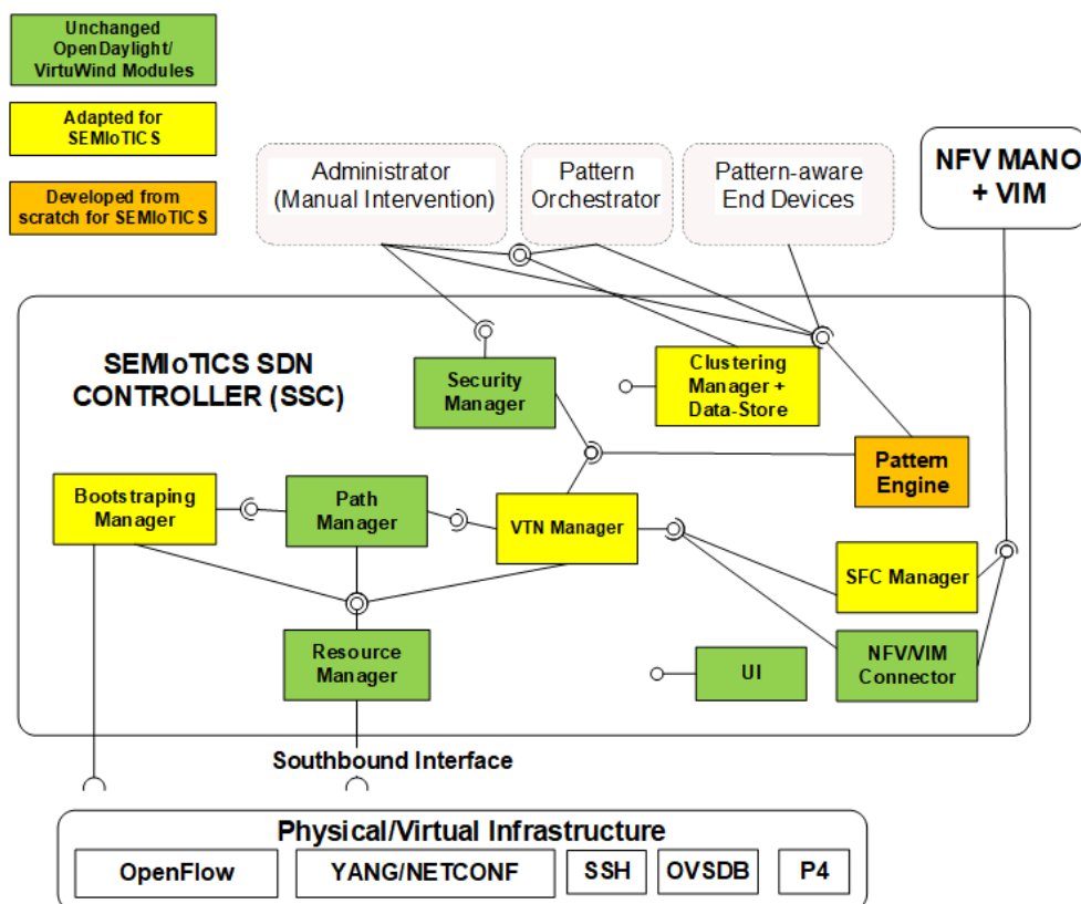
FIGURE 5: SEMIoTICS SDN CONTROLLER ARCHITECTURE
