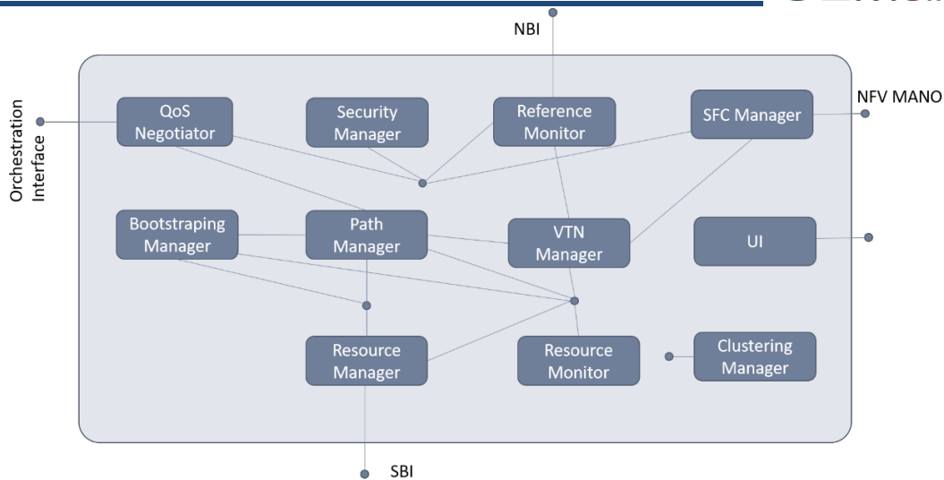
FIGURE 6: COMPONENT OVERVIEW OF THE VIRTUWIND SDN CONTROLLER
