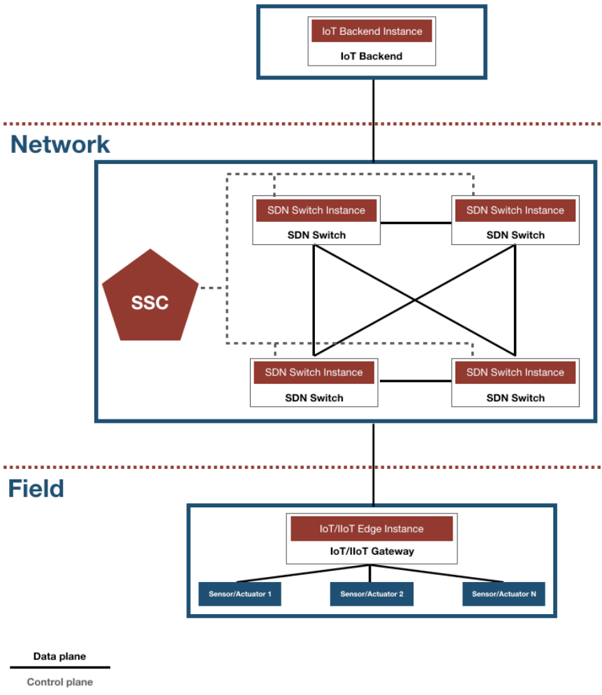
FIGURE 2: INSTANCE OF THE SEMIoTICS ARCHITECTURE DEPLOYMENT VIEW
