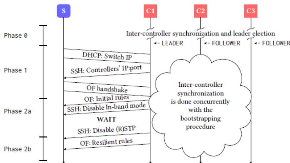
FIGURE 7: HSW - MESSAGE SEQUENCE DIAGRAM OF THE BOOTSTRAPPING PROCEDURE (VIRTUWIND STATE-OF-THE-ART)
