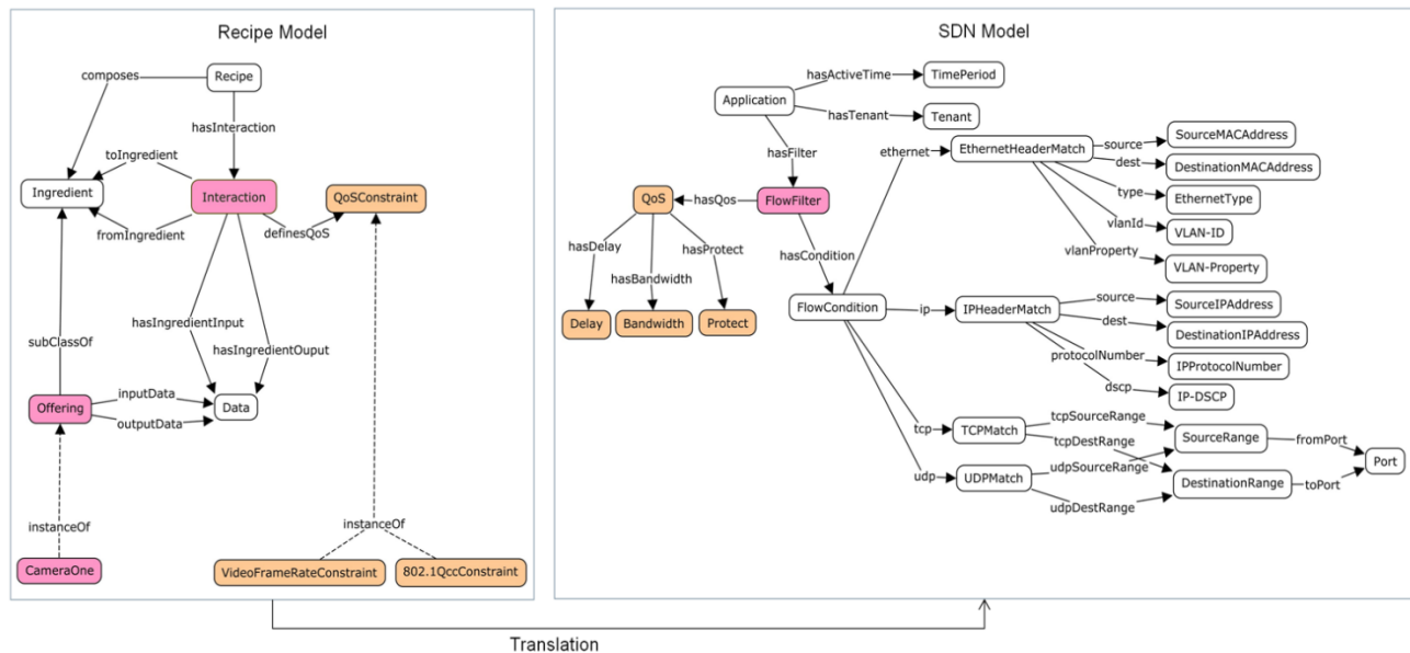
FIGURE 30. TRANSFORMATION FROM RECIPE TO NETWORK CONFIGURATION [43]
