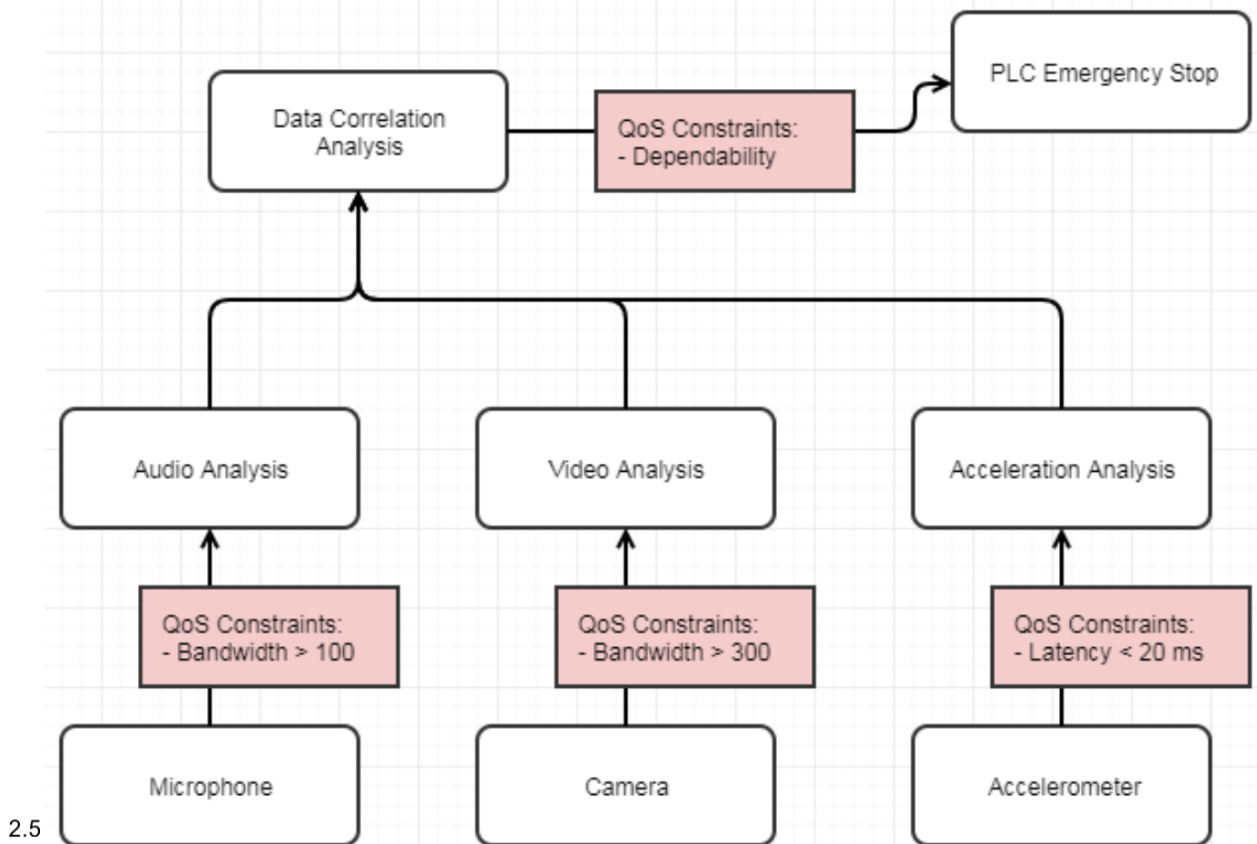
FIGURE 7. EXAMPLE OF A DATA FLOW BETWEEN IOT APPLICATIONS OF A WIND TURBINE
