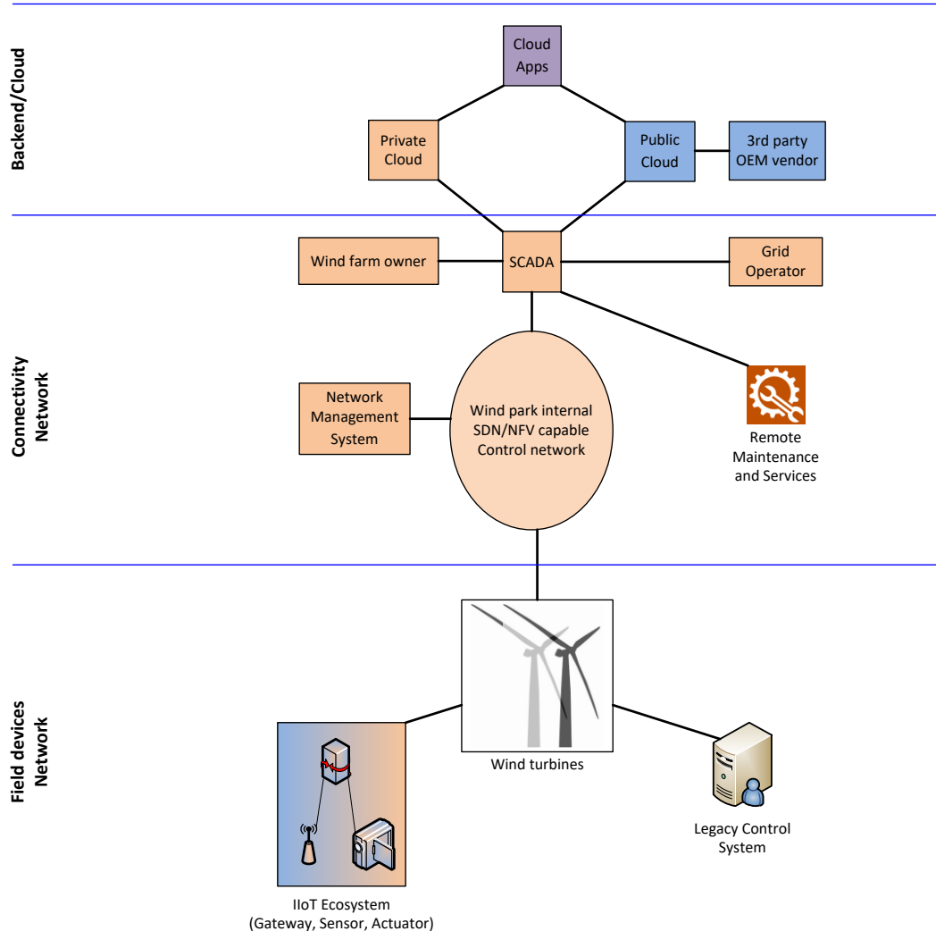
FIGURE 5. INTERACTIONS BETWEEN STAKEHOLDERS AT EACH LAYER IN THE IIOT WIND PARK SCENARIO
