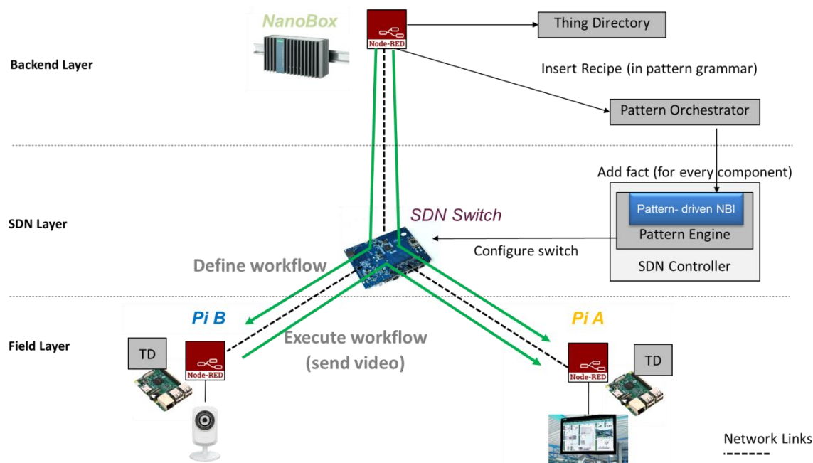
FIGURE 34. OIL LEAKAGE DETECTION APPLICATION SCENARIO (UC1)
