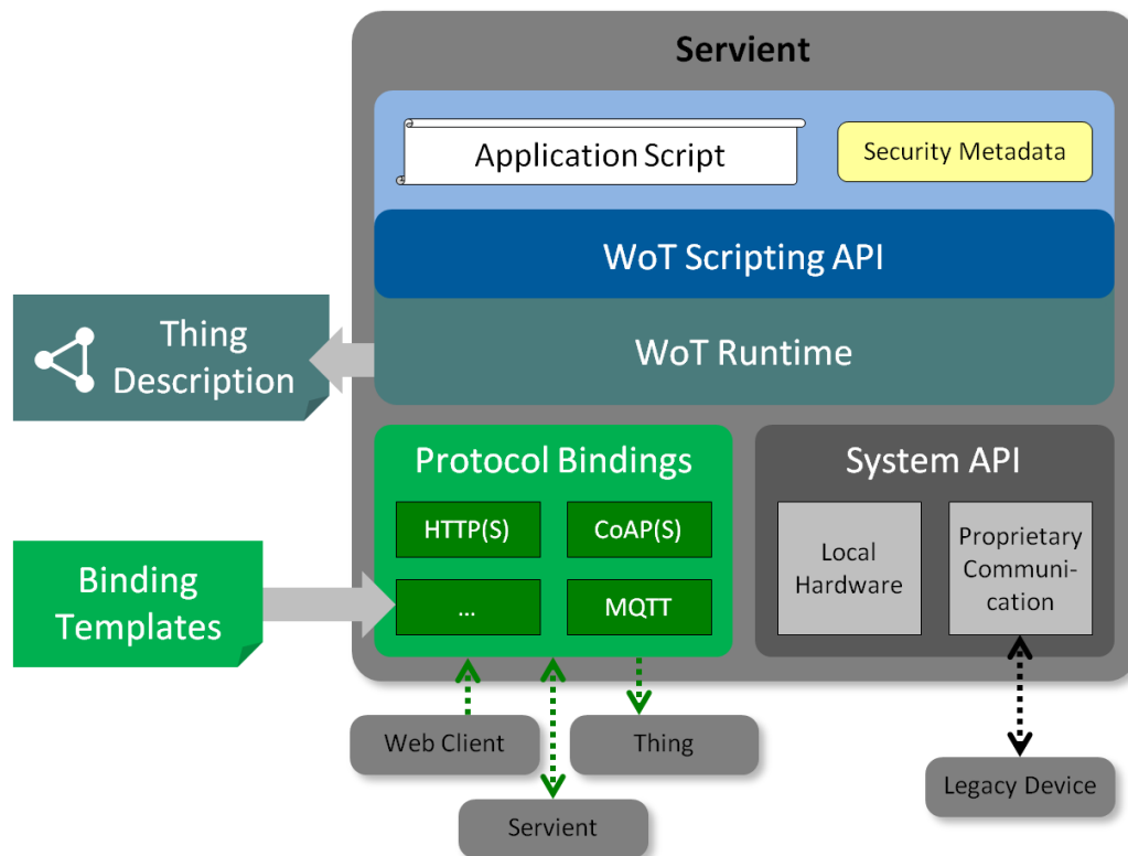
FIGURE 6. ARCHITECTURE FOR IOT APPLICATION EXECUTION USING W3C WEB OF THINGS [5]
