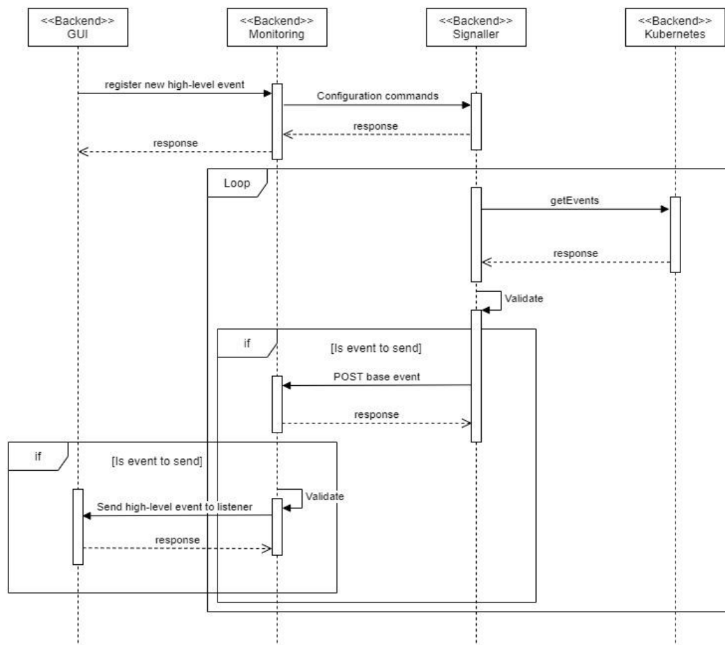
FIGURE 29 SEQUENCE DIAGRAM SHOWING THE FLOW BETWEEN COMPONENTS
