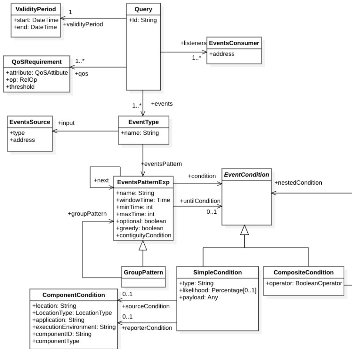
FIGURE 11 QUERIES OBJECT MODEL
