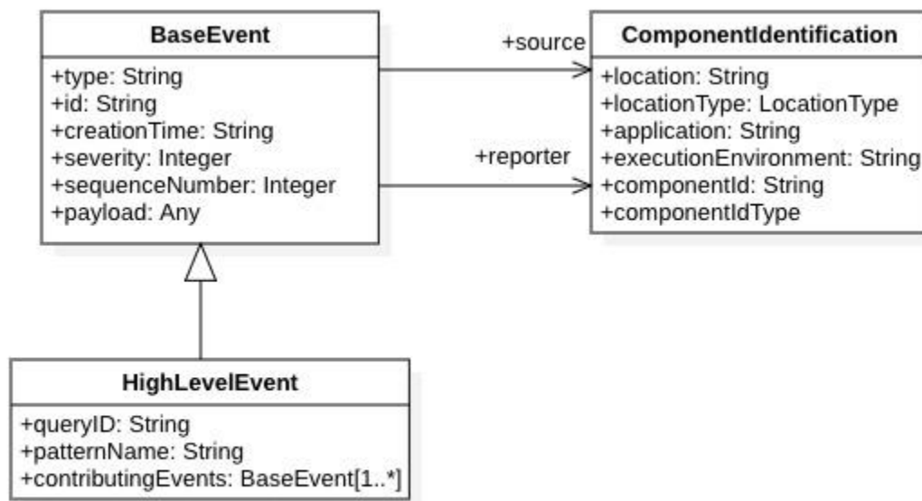
FIGURE 10 SEMIoTICS EVENT OBJECT MODEL
