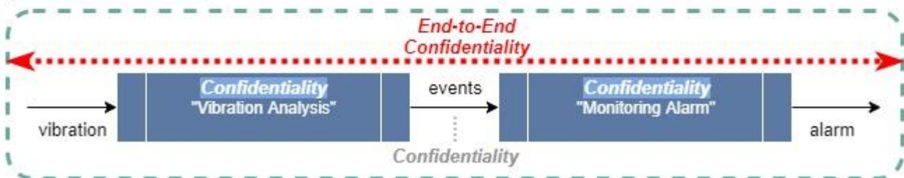
FIGURE 13 INSTANTIATED RECIPE (TOP) AND WORKFLOW (BOTTOM)
