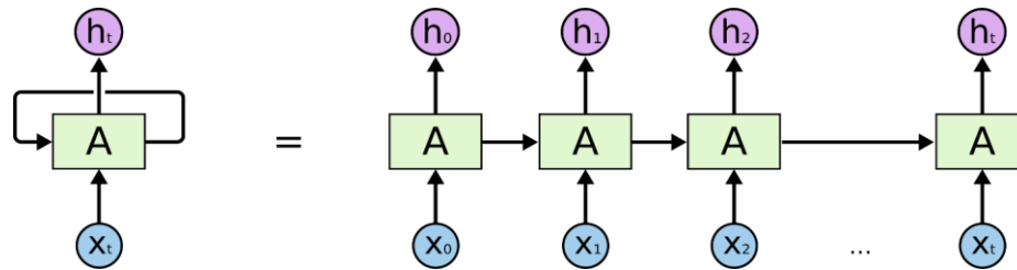
FIGURE 19 RNN UNROLLED- A TAKES AN INPUT x_t AND OUTPUTS A VALUE h_t [51]
