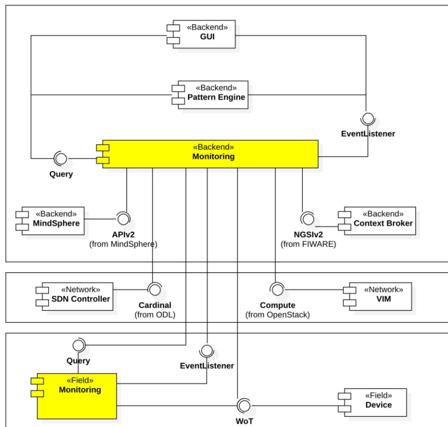
FIGURE 2 DEPENDENCIES OF THE MPD COMPONENT
