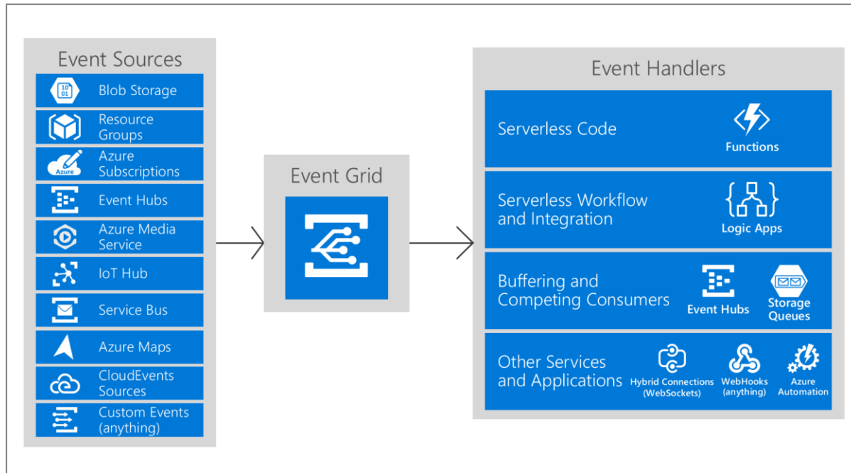
FIGURE 8 AZURE EVENT GRID SOURCES AND HANDLERS
