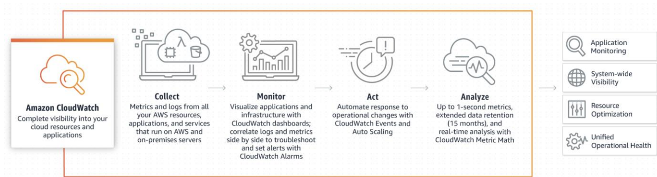
FIGURE 7 AWS CLOUDWATCH 4
